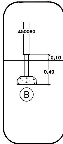
Sunken Foundation
